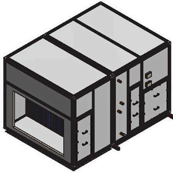
VIEW ISO 1 (1 : 38)
